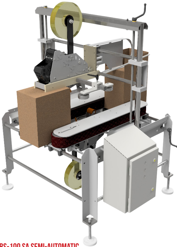
TBS-100 SA SEMI-AUTOMATIC Sanitary Top & Bottom Case Sealer with Leg Extensions
